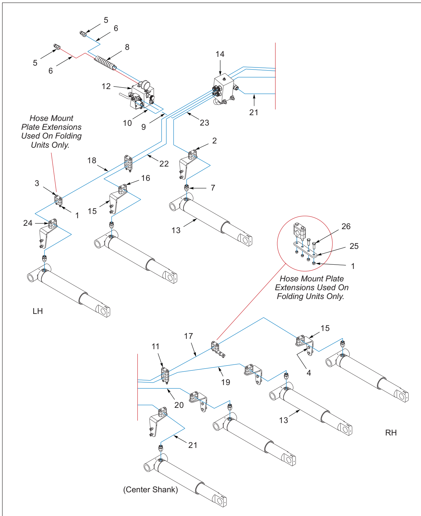
Figure 4-7: 2512 Hydraulics, 7 Shank (Rigid and Folding)
