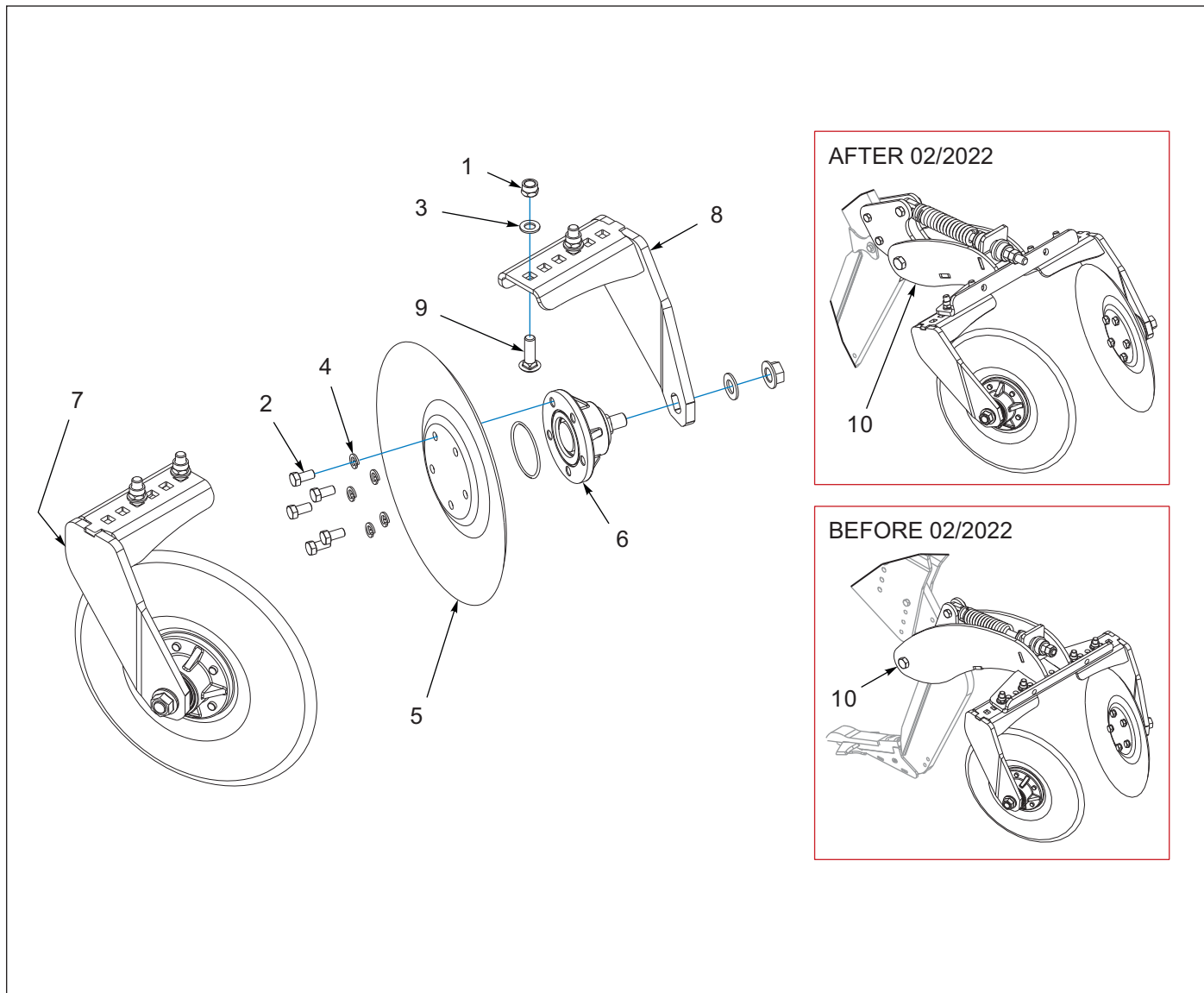
Figure 7-9: Closer Disc
