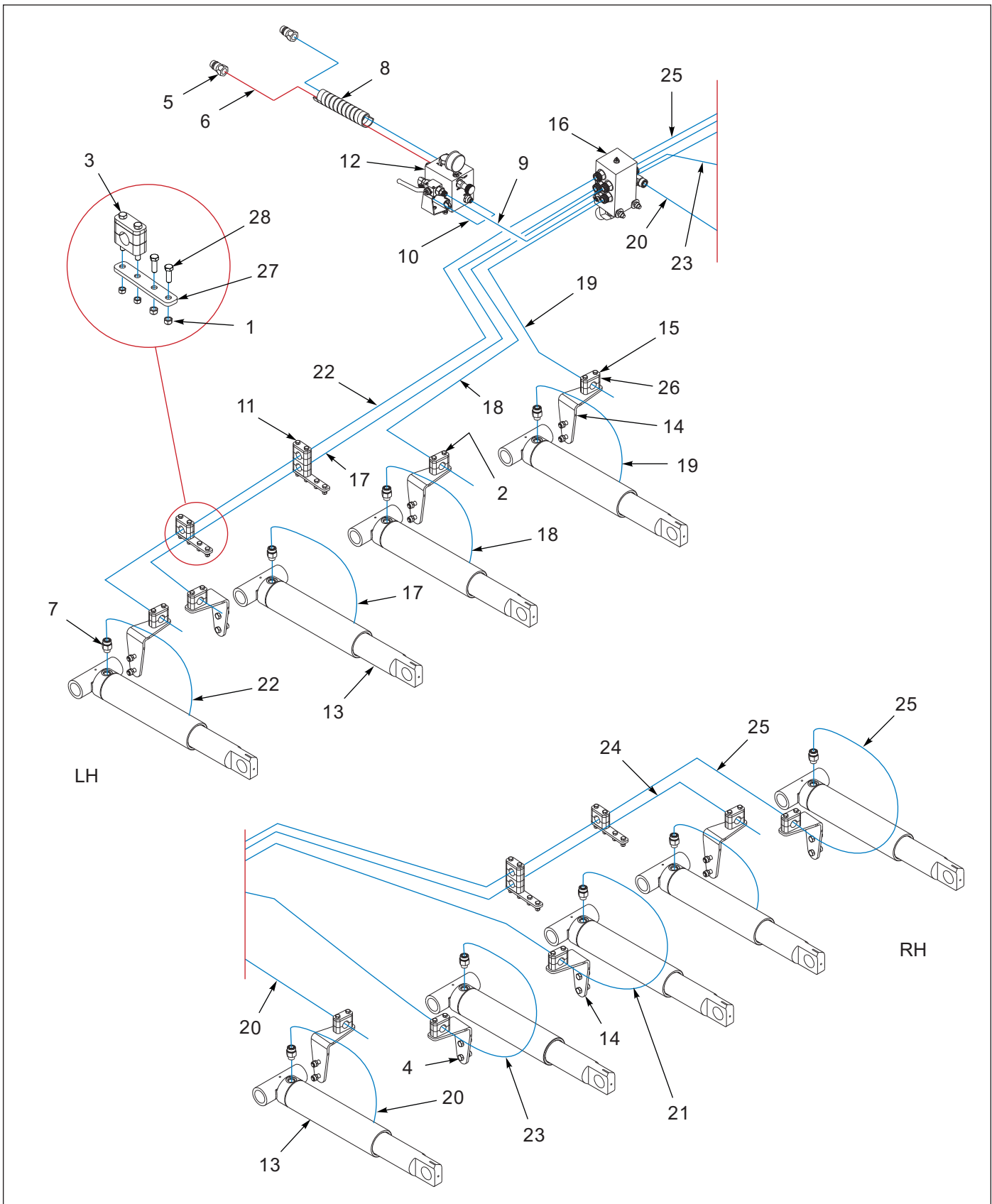
Figure 4-9: 2512 Hydraulics, 9 Shank (Folding) (1 of 2)
