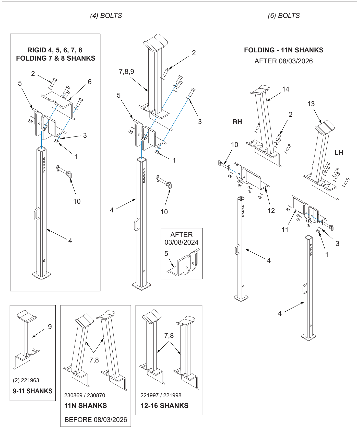
Figure 1-18: 2512 Jack Stand and Wing Rest (AFTER 06/07/2023)
