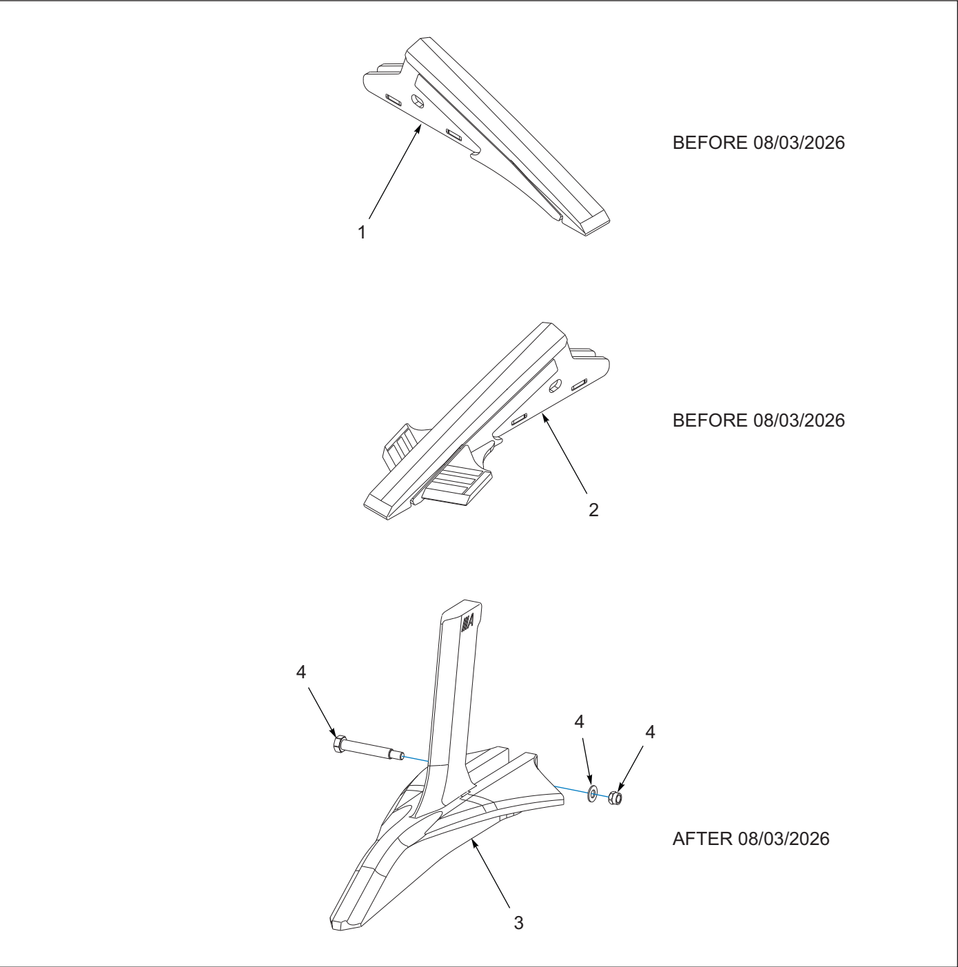
Figure 6-2: Points 3/4 Shank
