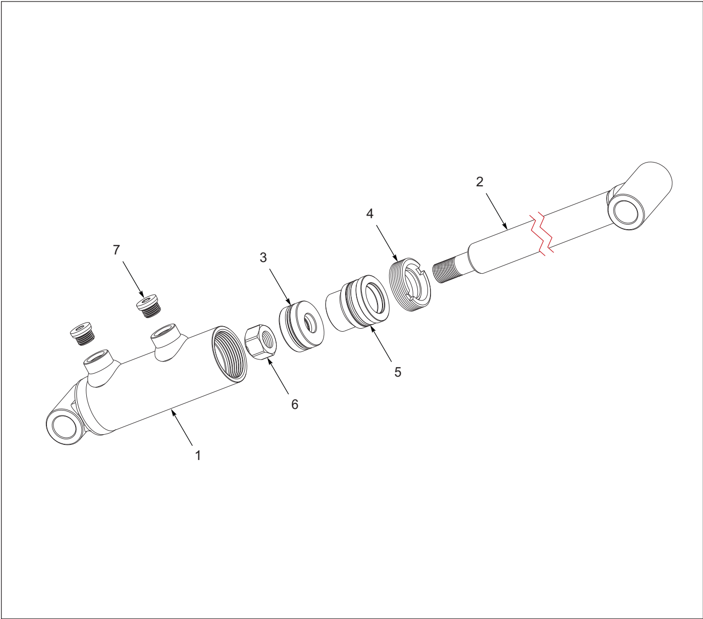
Figure 4-13: Hydraulic Cylinder, 1-1/2 x 1-1/2 - 230890
