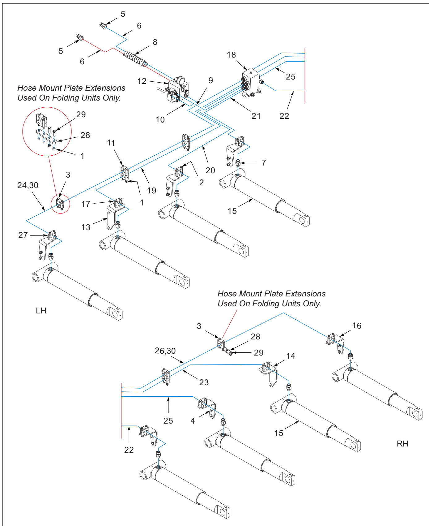
Figure 4-8: 2512 Hydraulics, 8 Shank (Rigid and Folding) (1 of 2)
