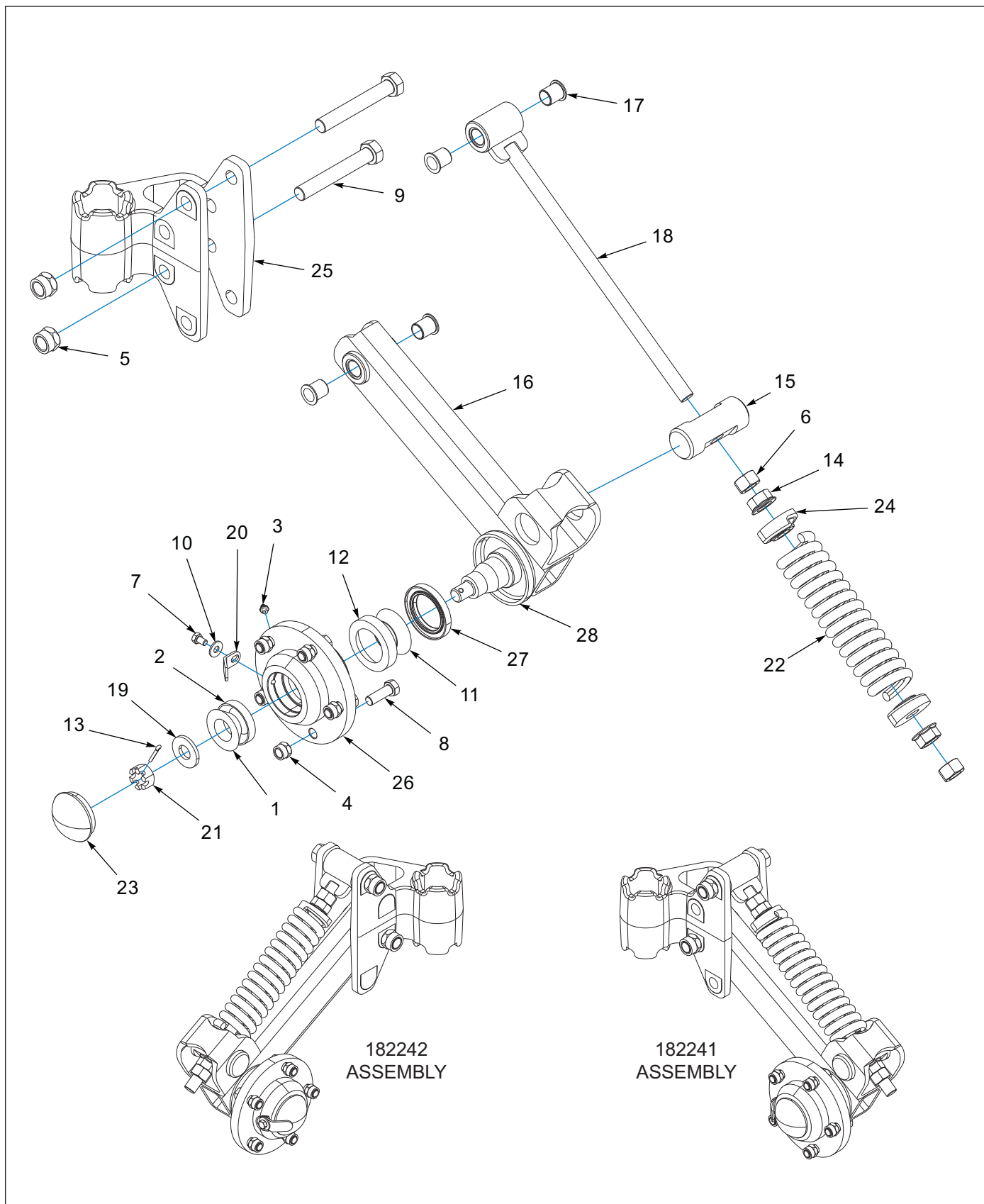
Figure 2-4: Heavy Duty Coulter (BEFORE 02/2022)
