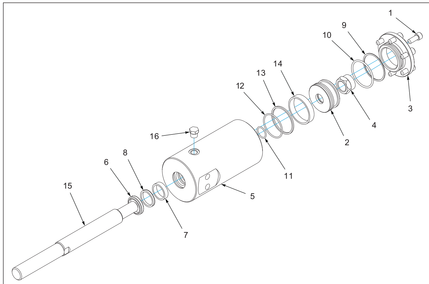
Figure 6-26: Cylinder Assembly 2-1/2 x 3-1/2
