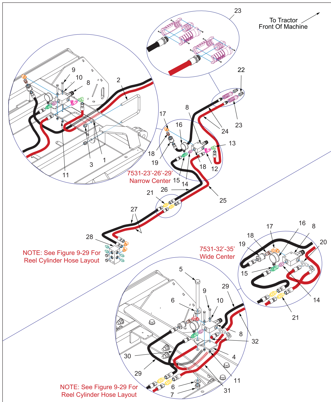
Figure 9-32: Live Reel Hydraulic Assembly
