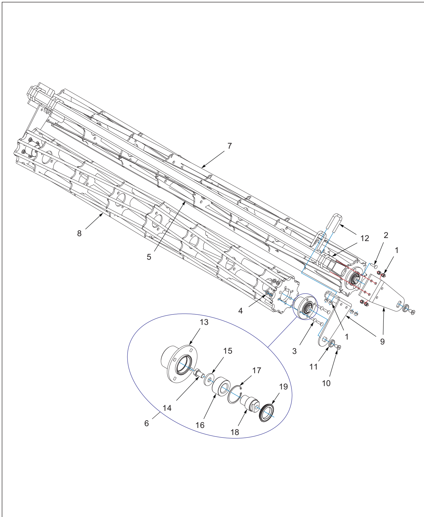
Figure 9-23: Double Flat/RD Reel Assembly 7531-23'-29' Center
