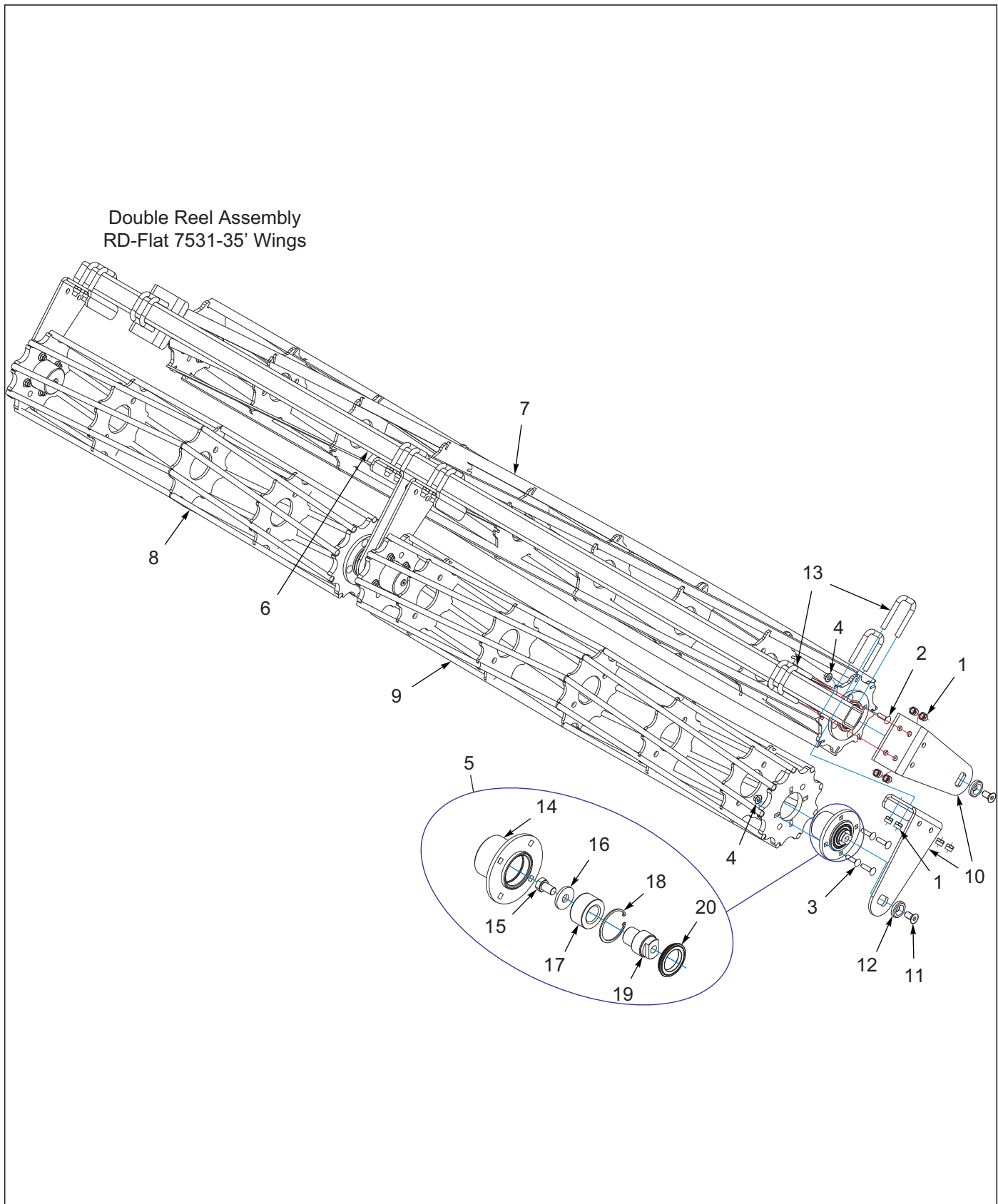
Figure 9-29: Double Flat/RD Reel Assembly 7531-35' Wings
