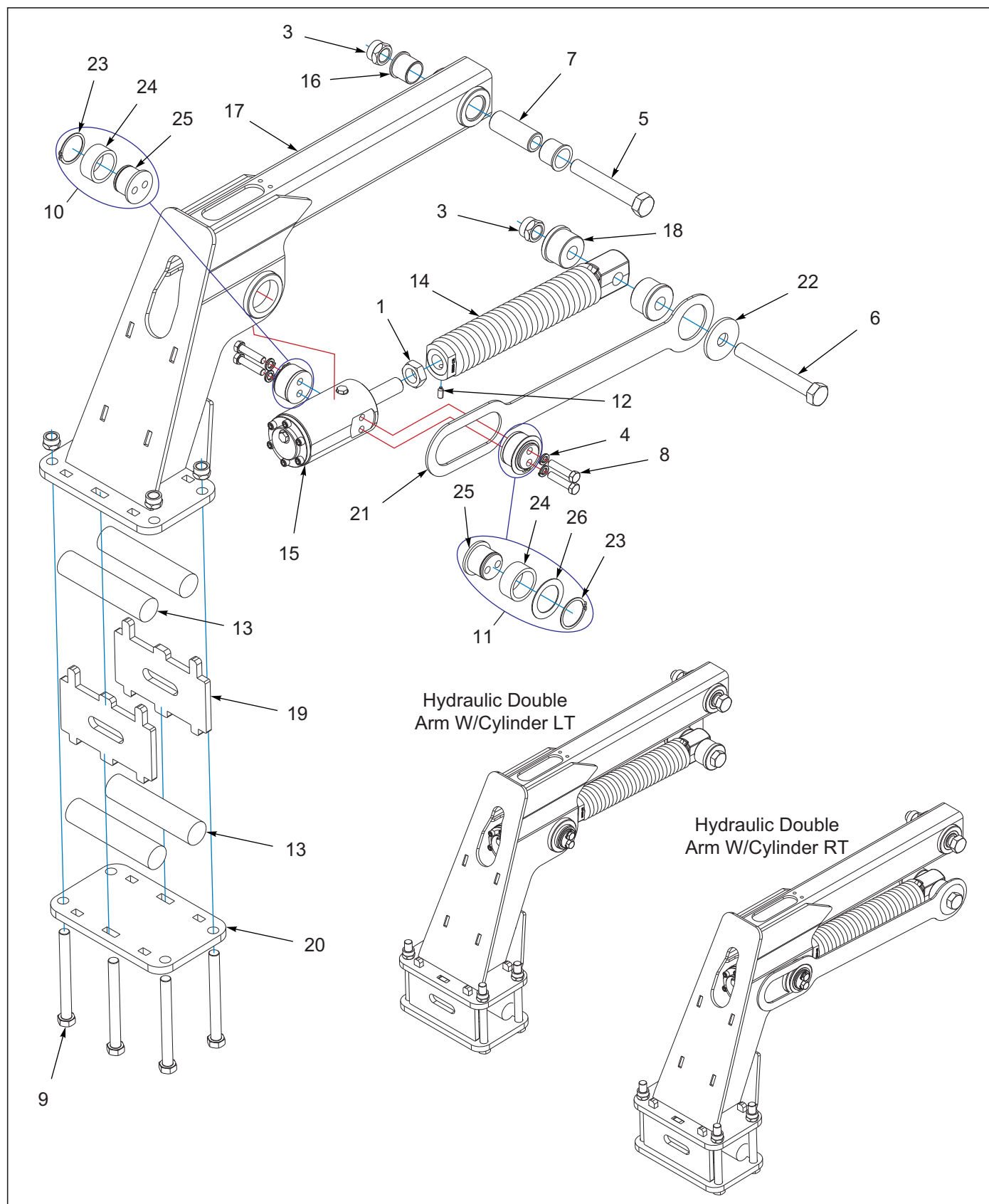
Figure 9-19: Hydraulic Double Arm W/Stop Assembly
