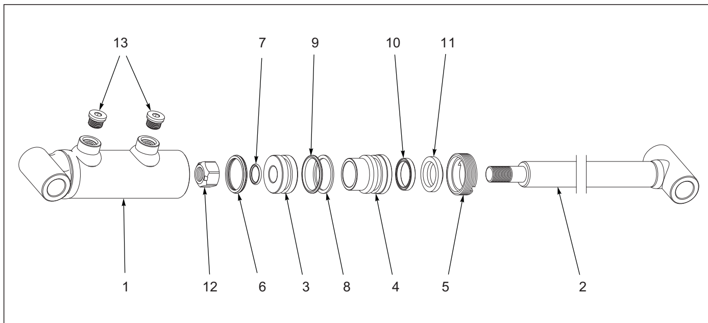
Figure 6-27: Cylinder Assembly 1-1/2 x -1-1/2
