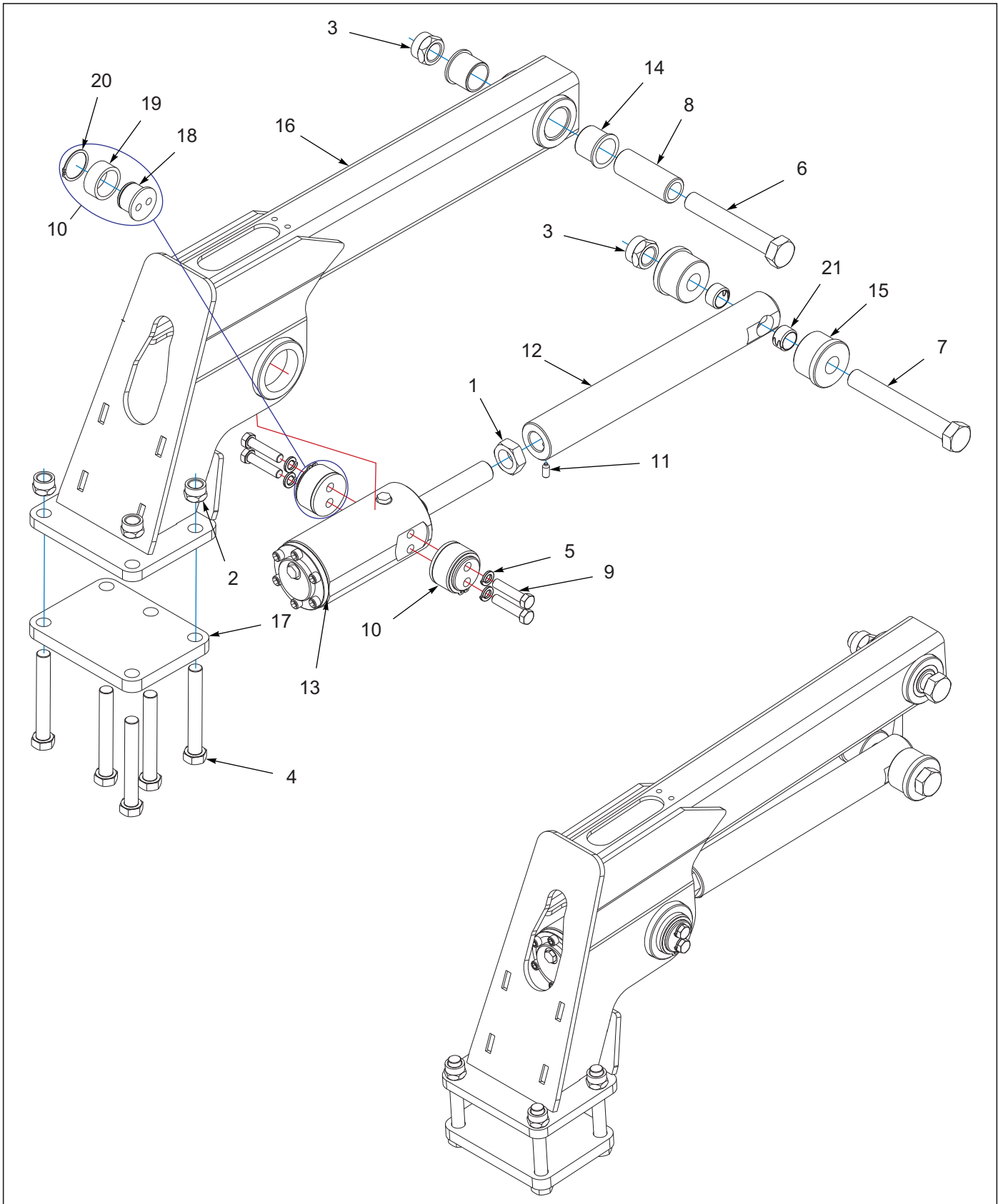
Figure 9-13: Live Hydraulic Single Arm Assembly
