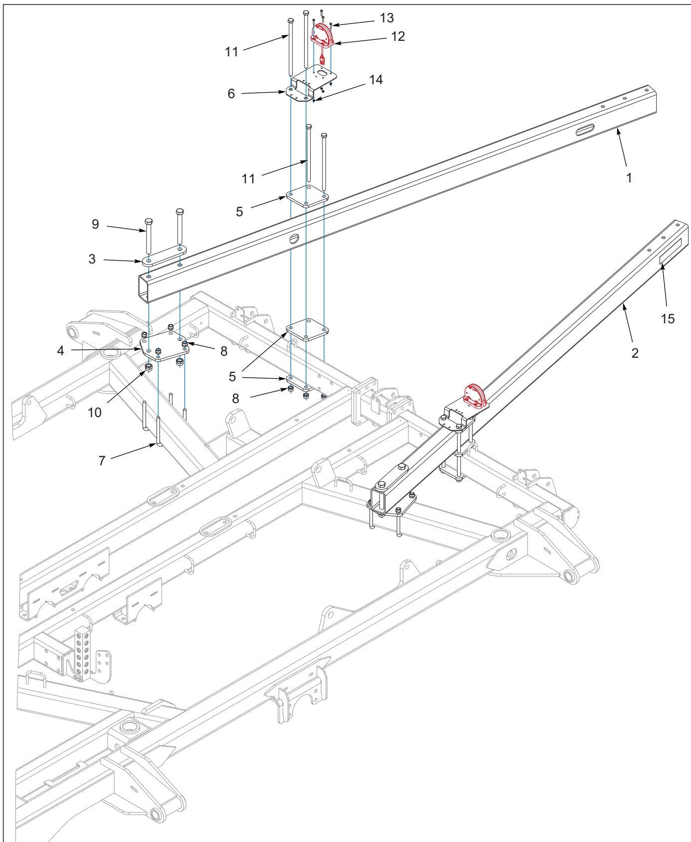
Figure 9-36: Rear Tow Assembly 7531-32'-35' (1 of 2)
