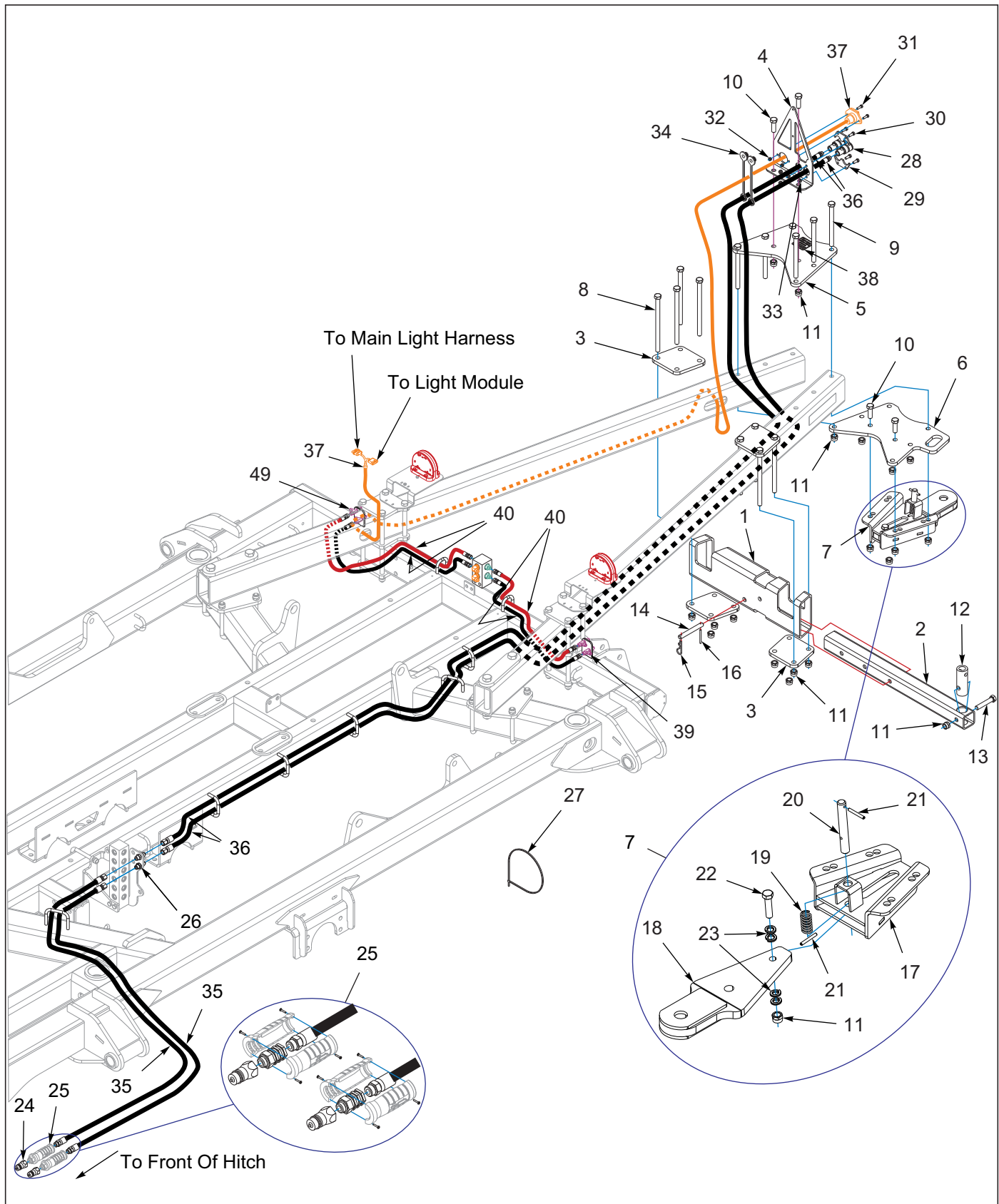
Figure 9-35: Rear Tow Assembly 7531-23'-26'-29' (2 of 2)
