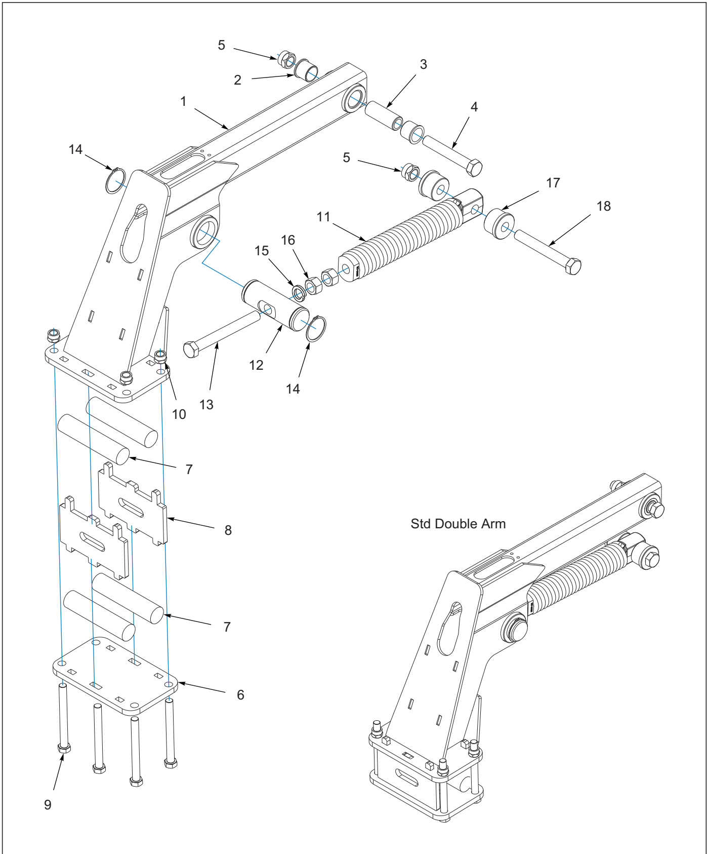
Figure 9-15: Std Double Arm Assembly
