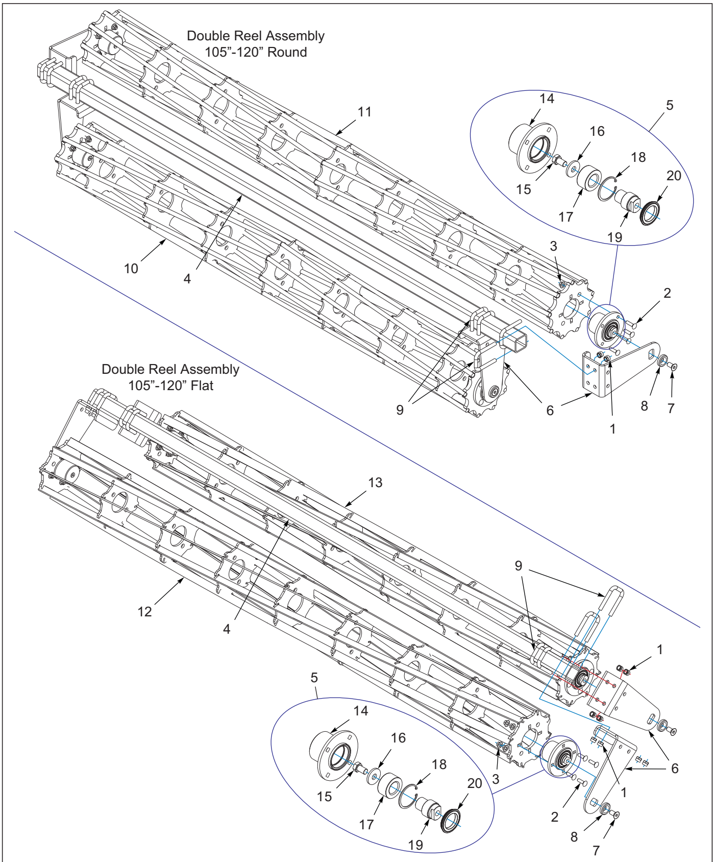
Figure 9-21: Double Reel Assembly 7531-23'-29' Center
