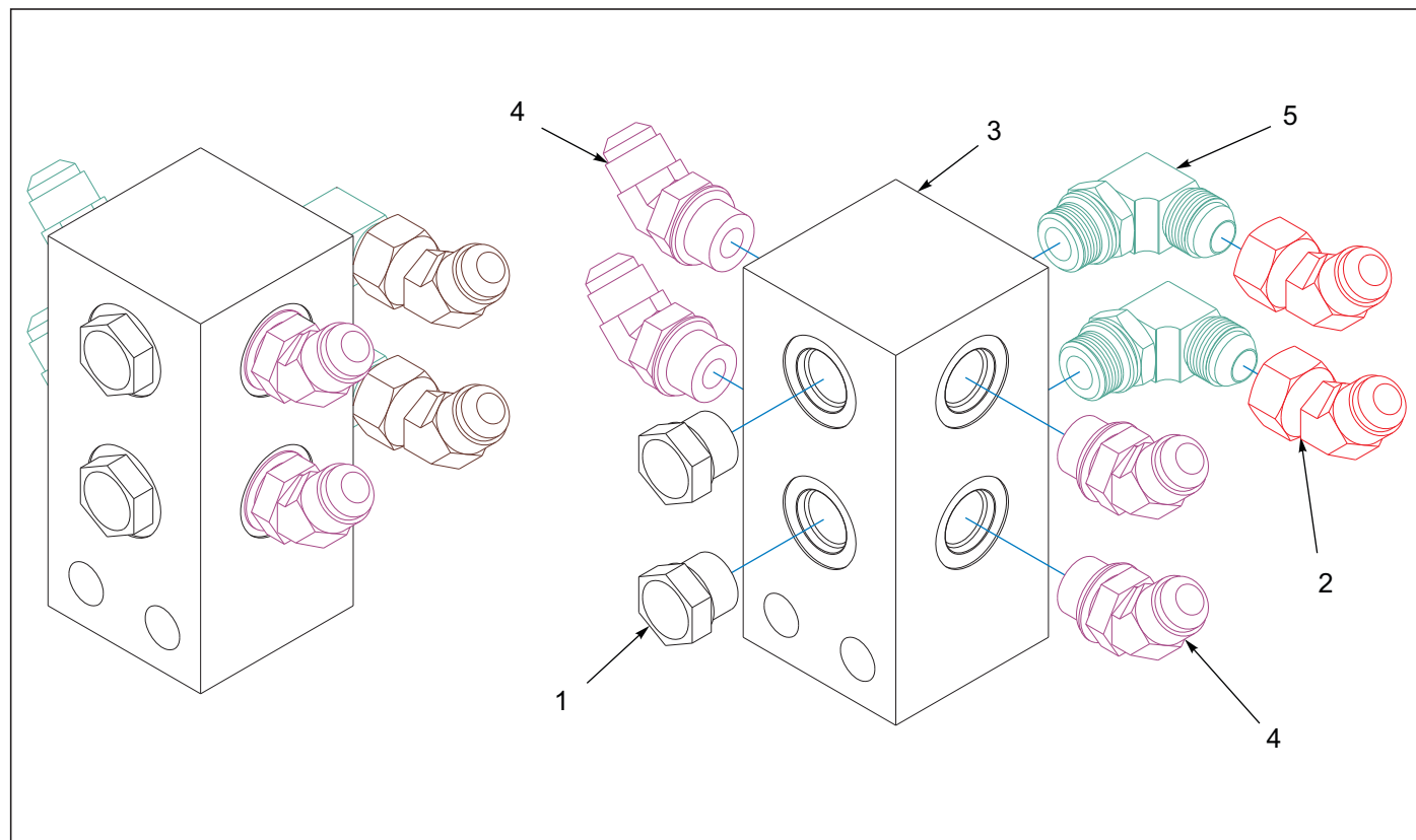
Figure 5-31: Manifold Assembly Front 7531-32'-35'
