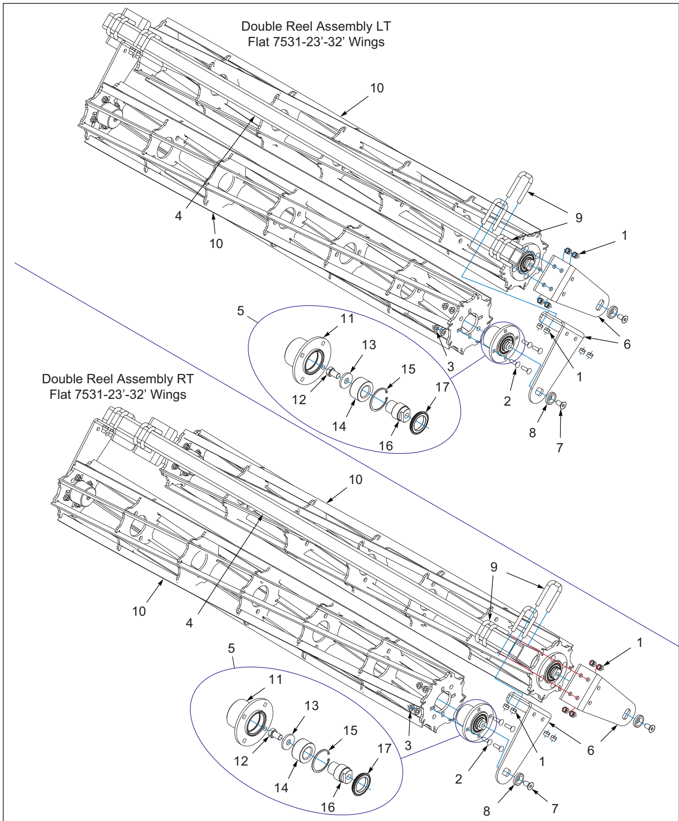
Figure 9-26: Double Flat Reel Assembly 7531-23'-32' Wings
