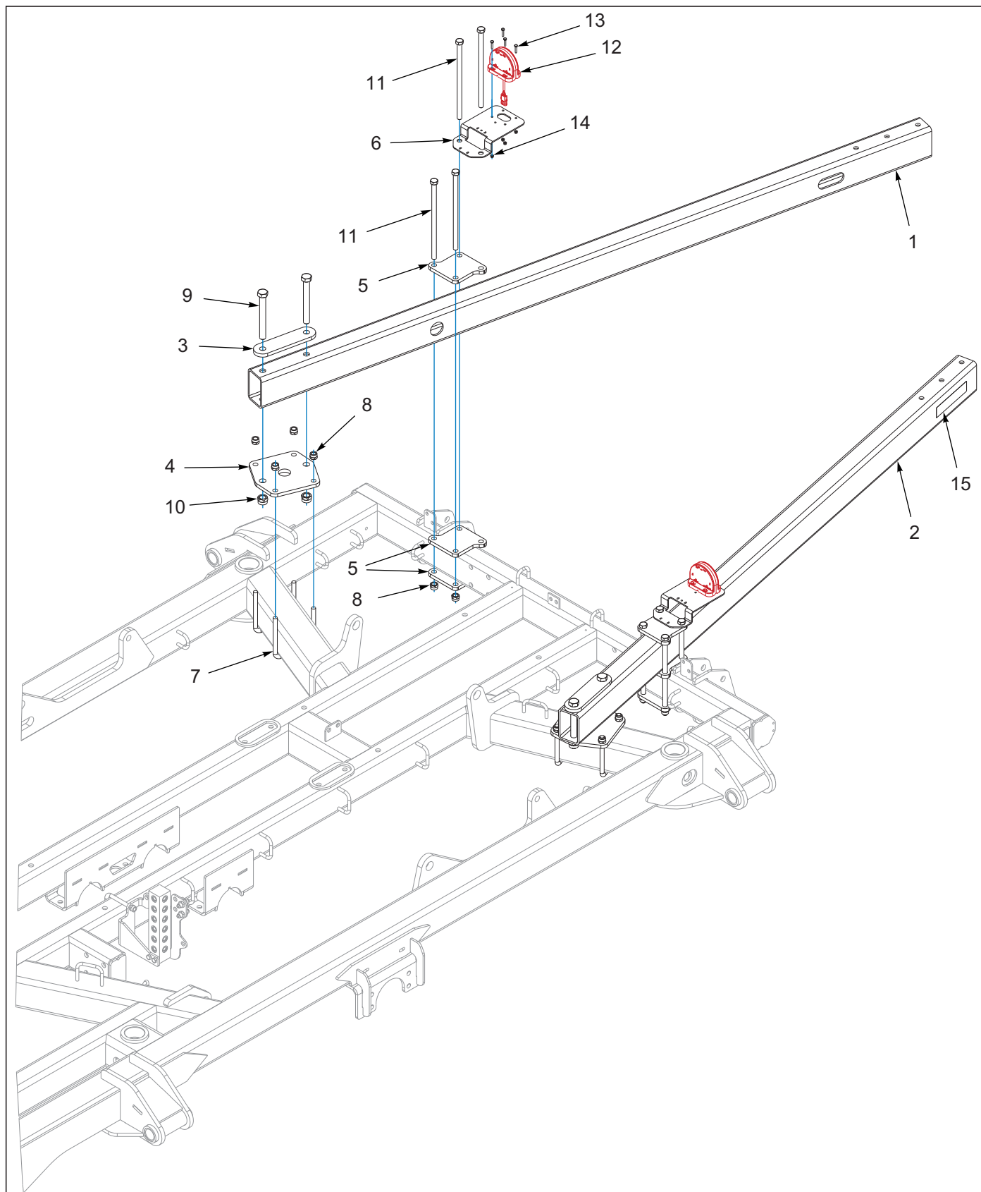
Figure 9-34: Rear Tow Assembly 8531-23'-26'-29' (1 of 2)
