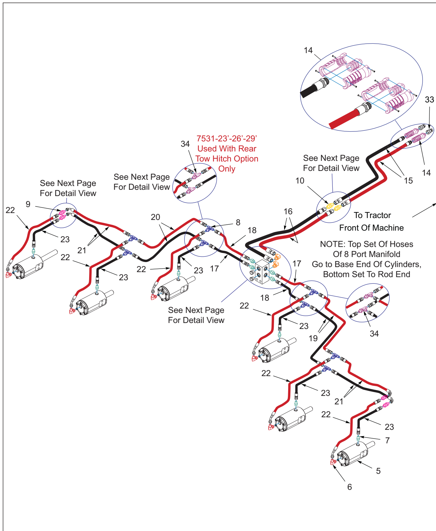
Figure 9-30: Reel Hydraulic Assembly (1 of 2)
