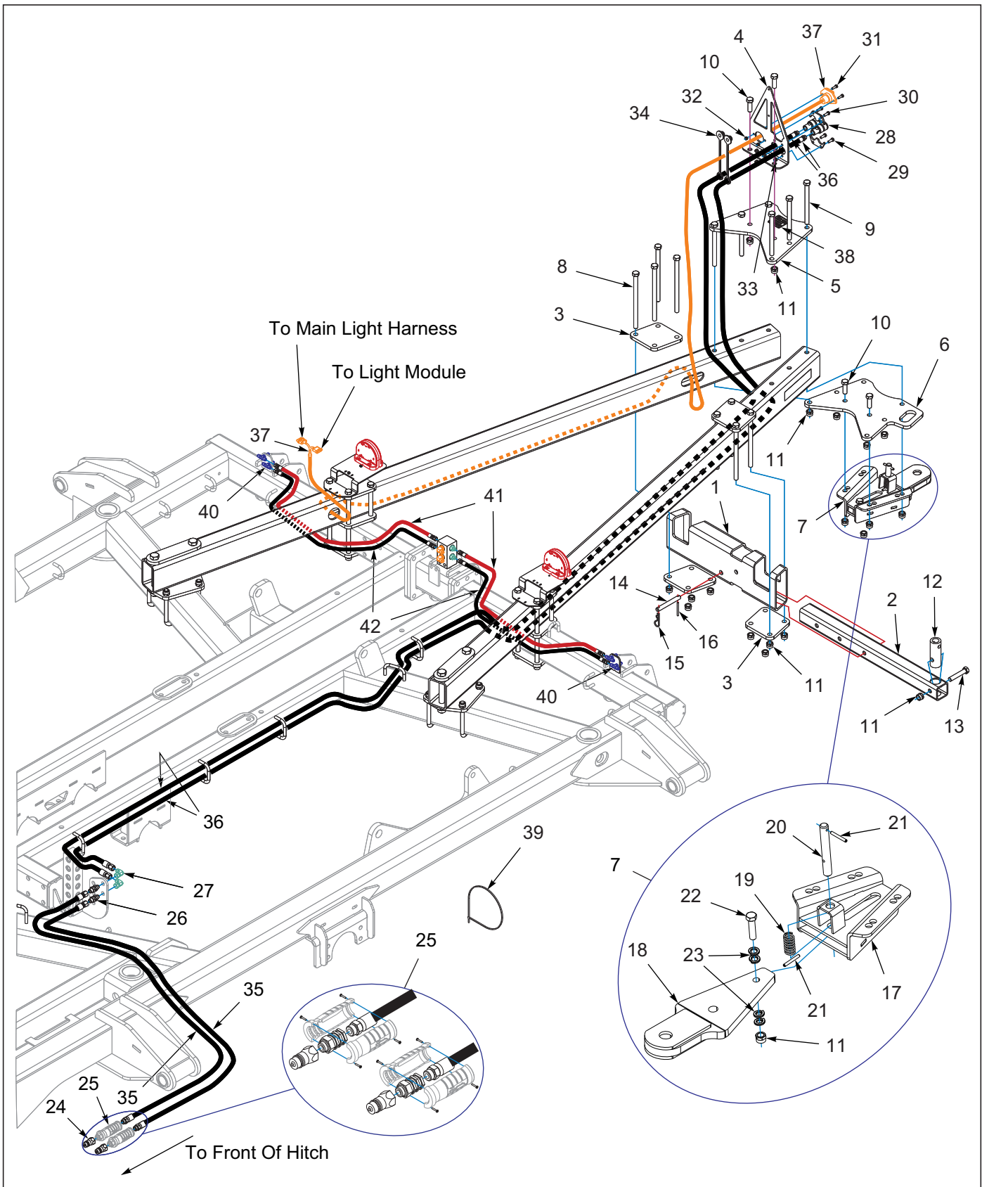
Figure 9-37: Rear Tow Assembly 7531-32'-35' (2 of 2)
