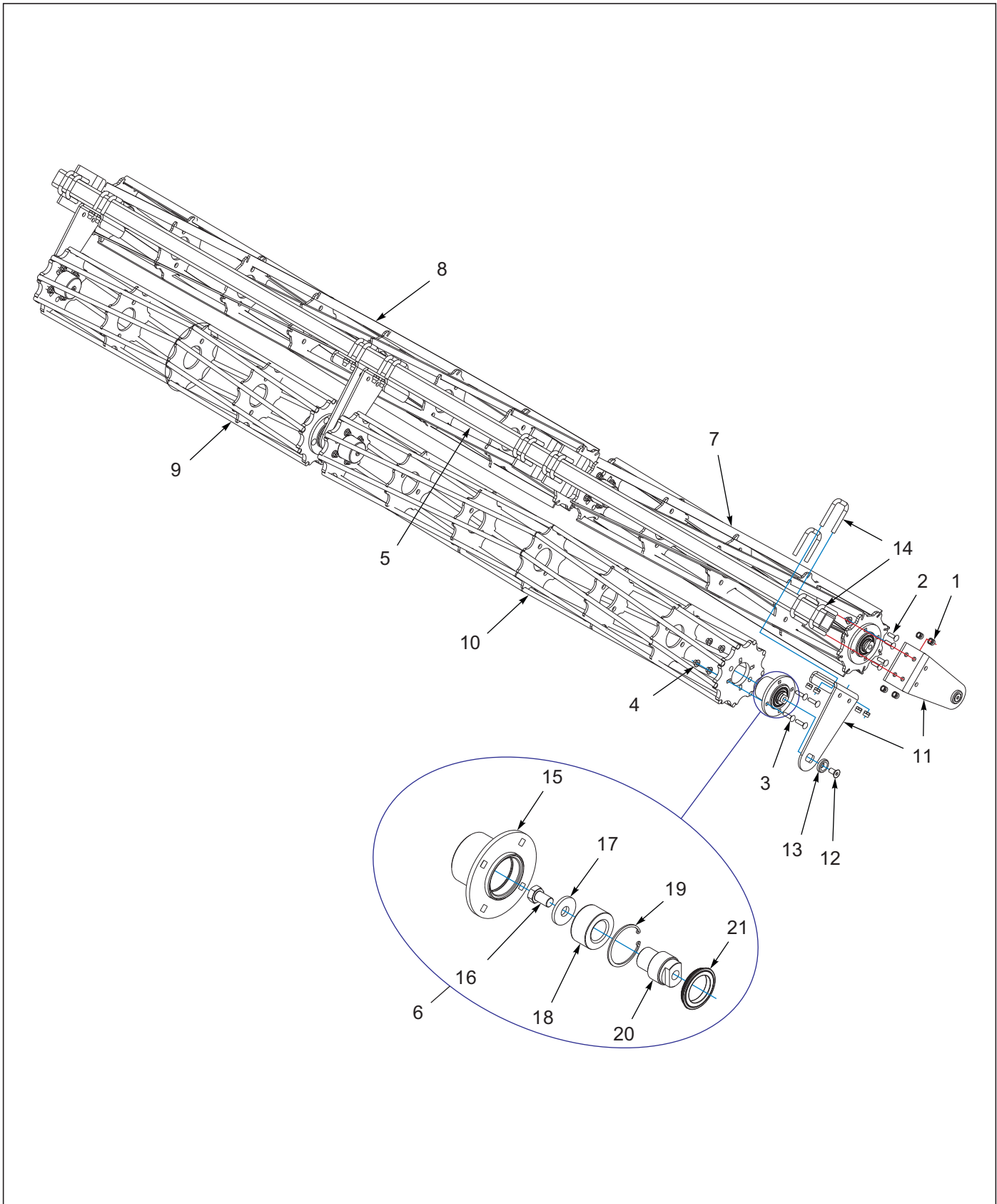
Figure 9-24: Double Flat/RD Reel Assembly 7531-32'-35' Center
