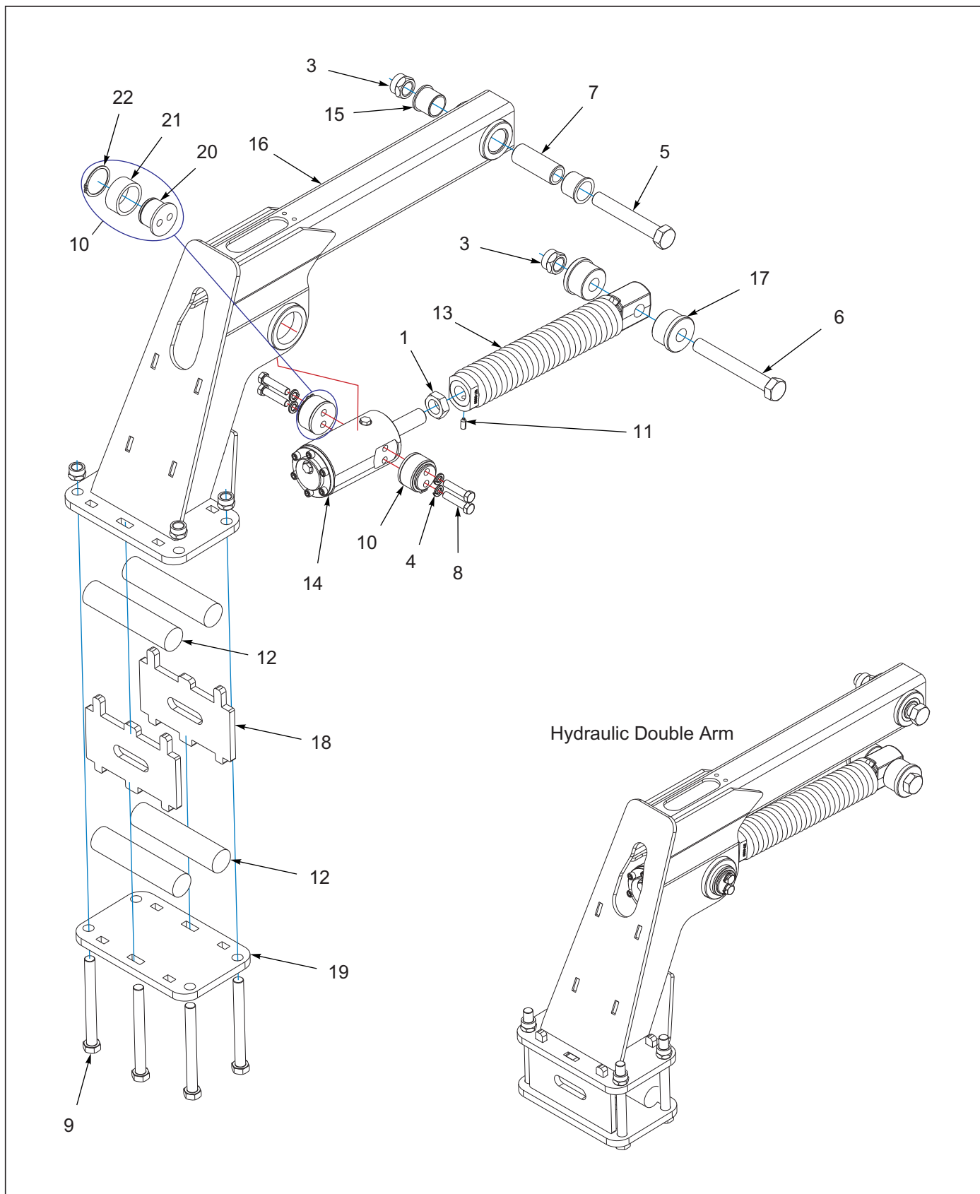
Figure 9-17: Hydraulic Double Arm Assembly
