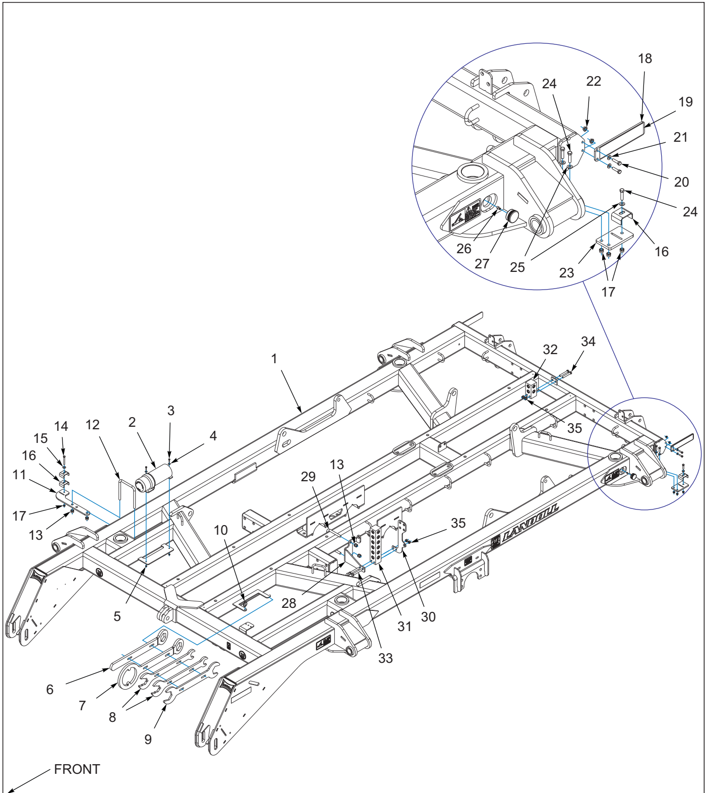
Figure 1-1: Frame Assembly 23'-26'-29'
