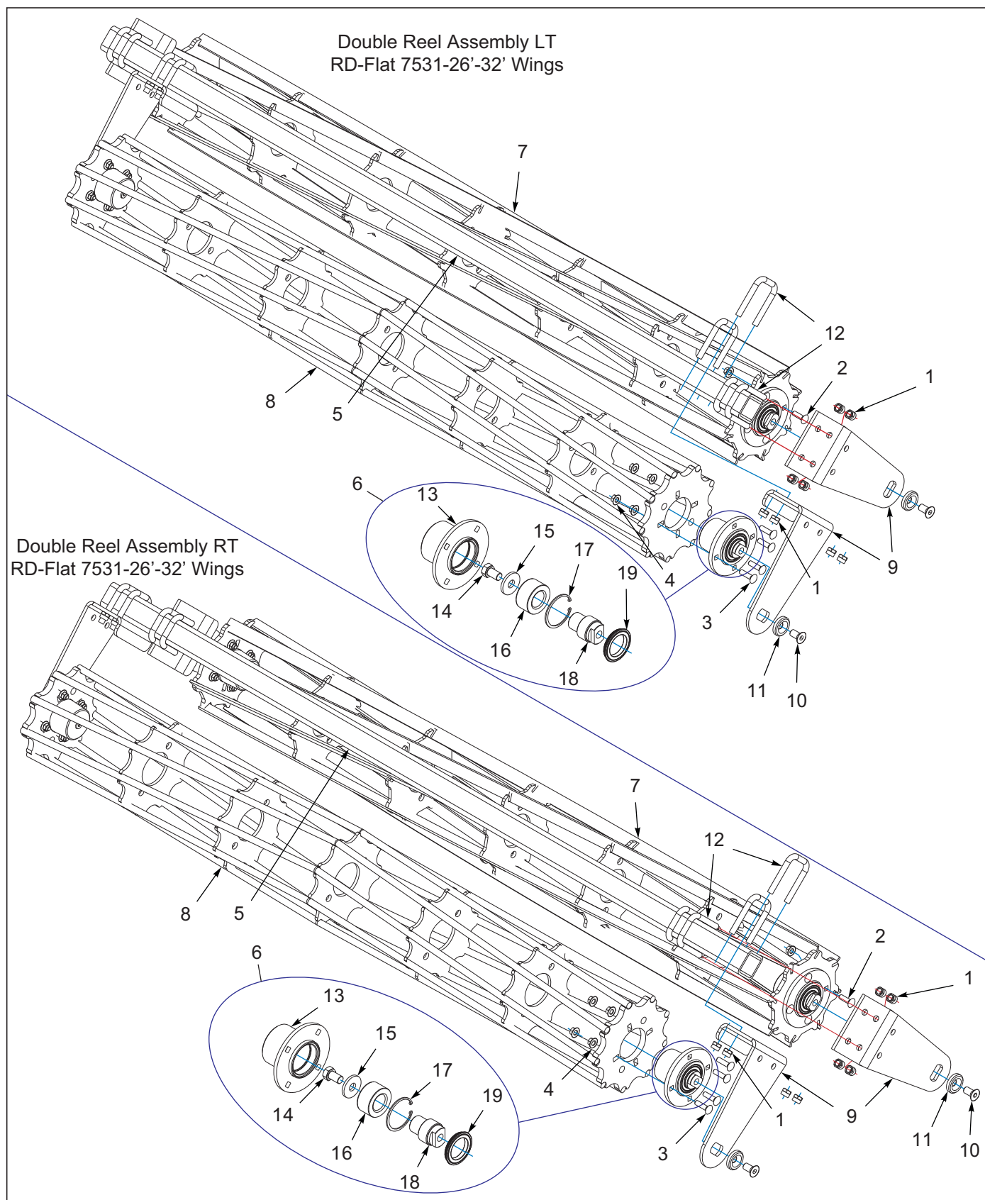
Figure 9-28: Double Flat/RD Reel Assembly 7531-23'-32' Wings
