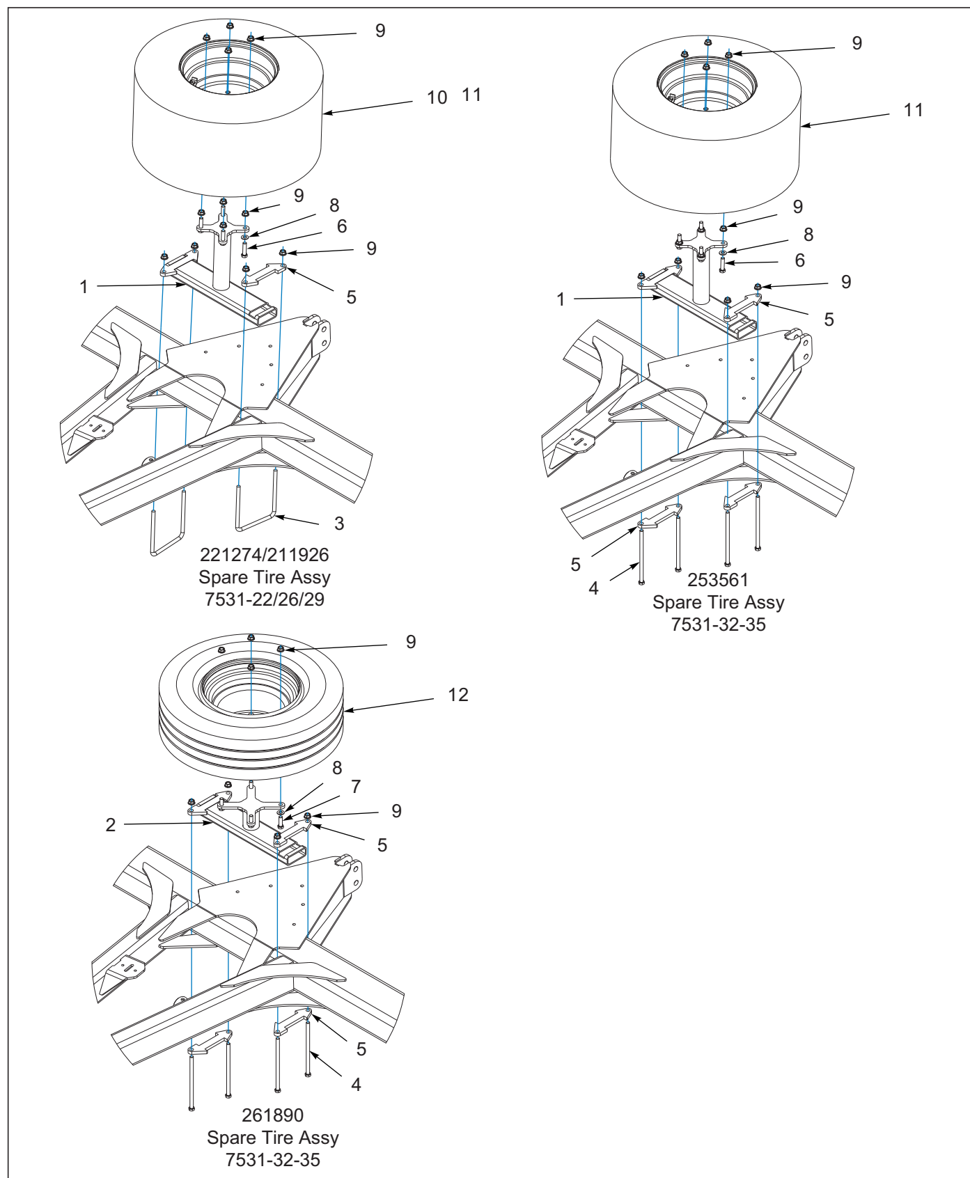
Figure 9-33: Spare Tire Assembly
