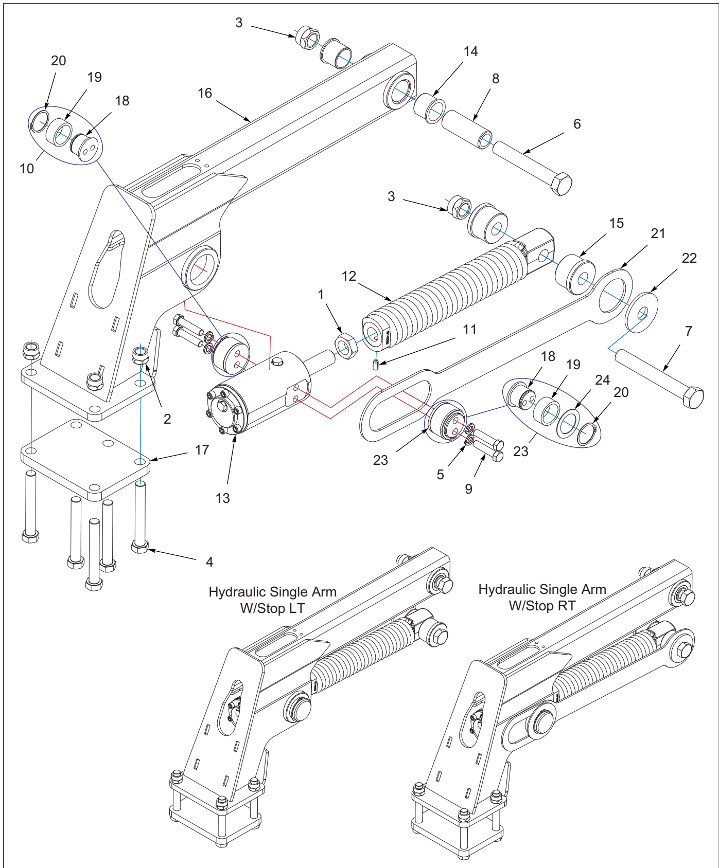
Figure 9-14: Hydraulic Single Arm W/Stop Assembly
