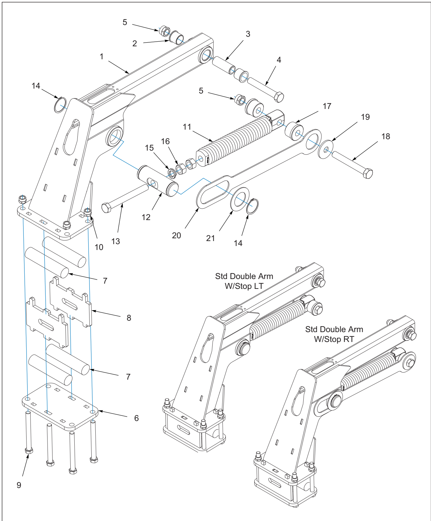
Figure 9-16: STD Double Arm W/Stop Assembly
