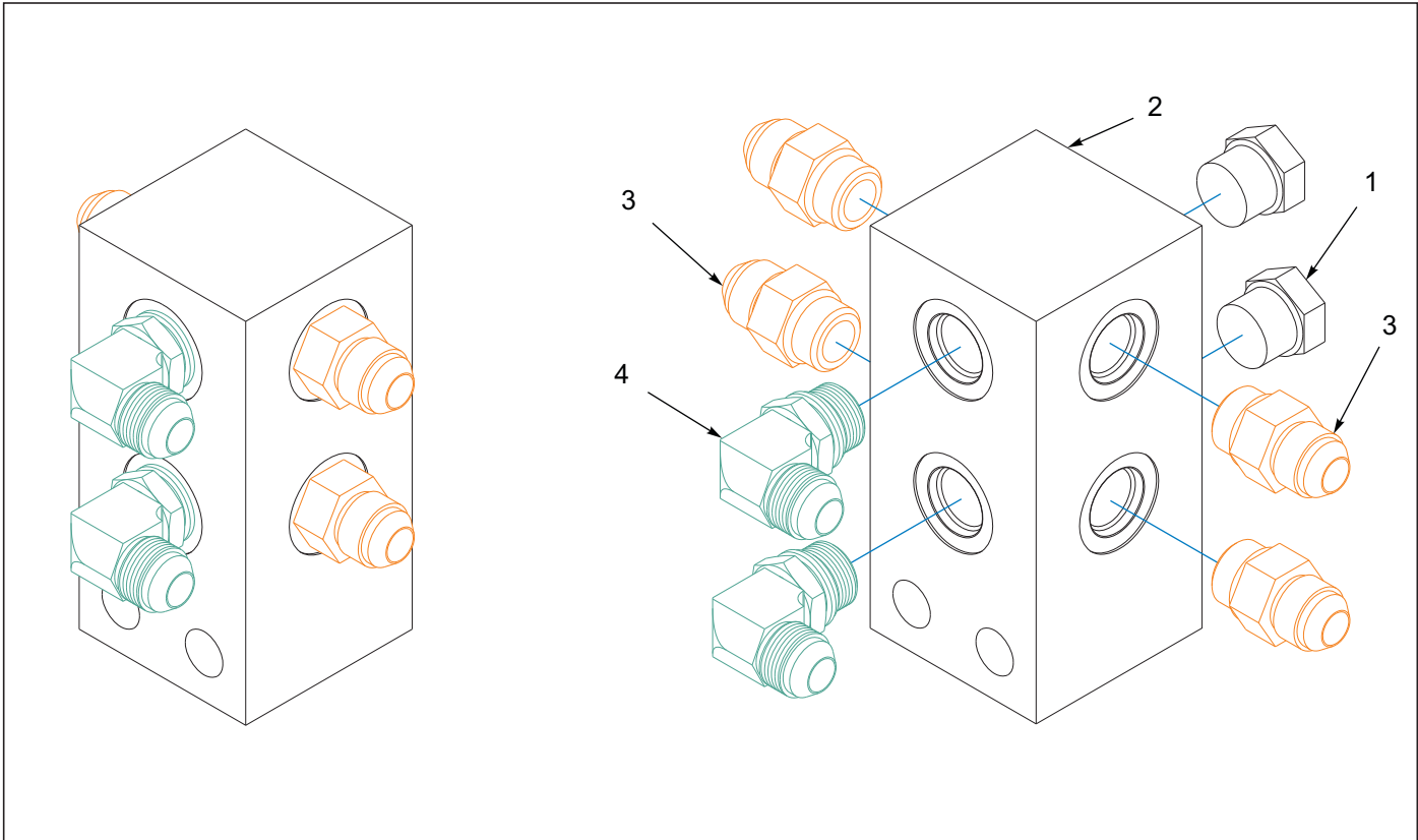
Figure 5-27: Manifold Assembly Front 7531-26'/29' (After S/N 75K2501921)
