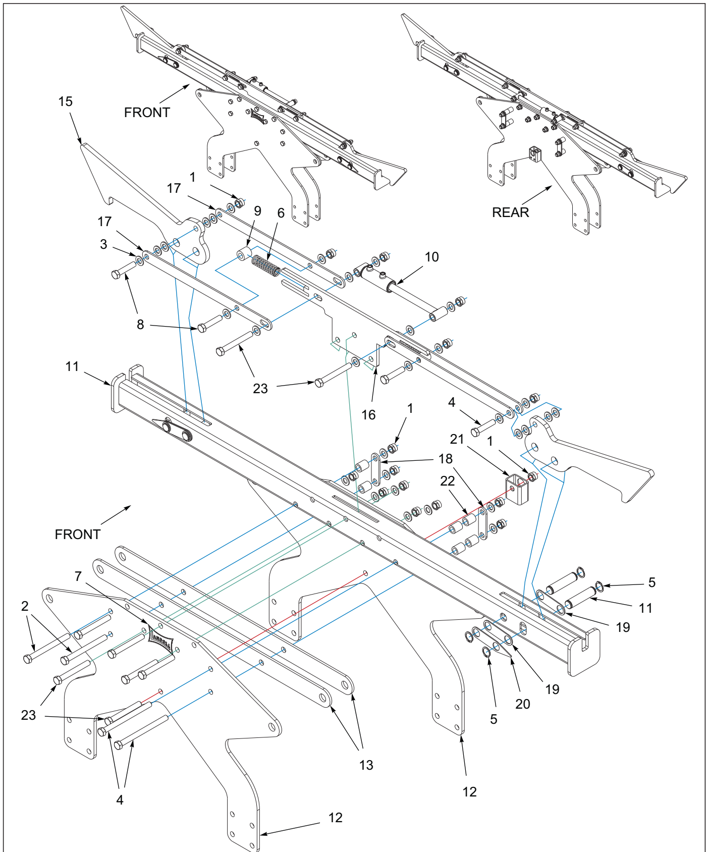
Figure 5-8: Wing Fold Stabilizer Assembly 7531-32'-35' Front
