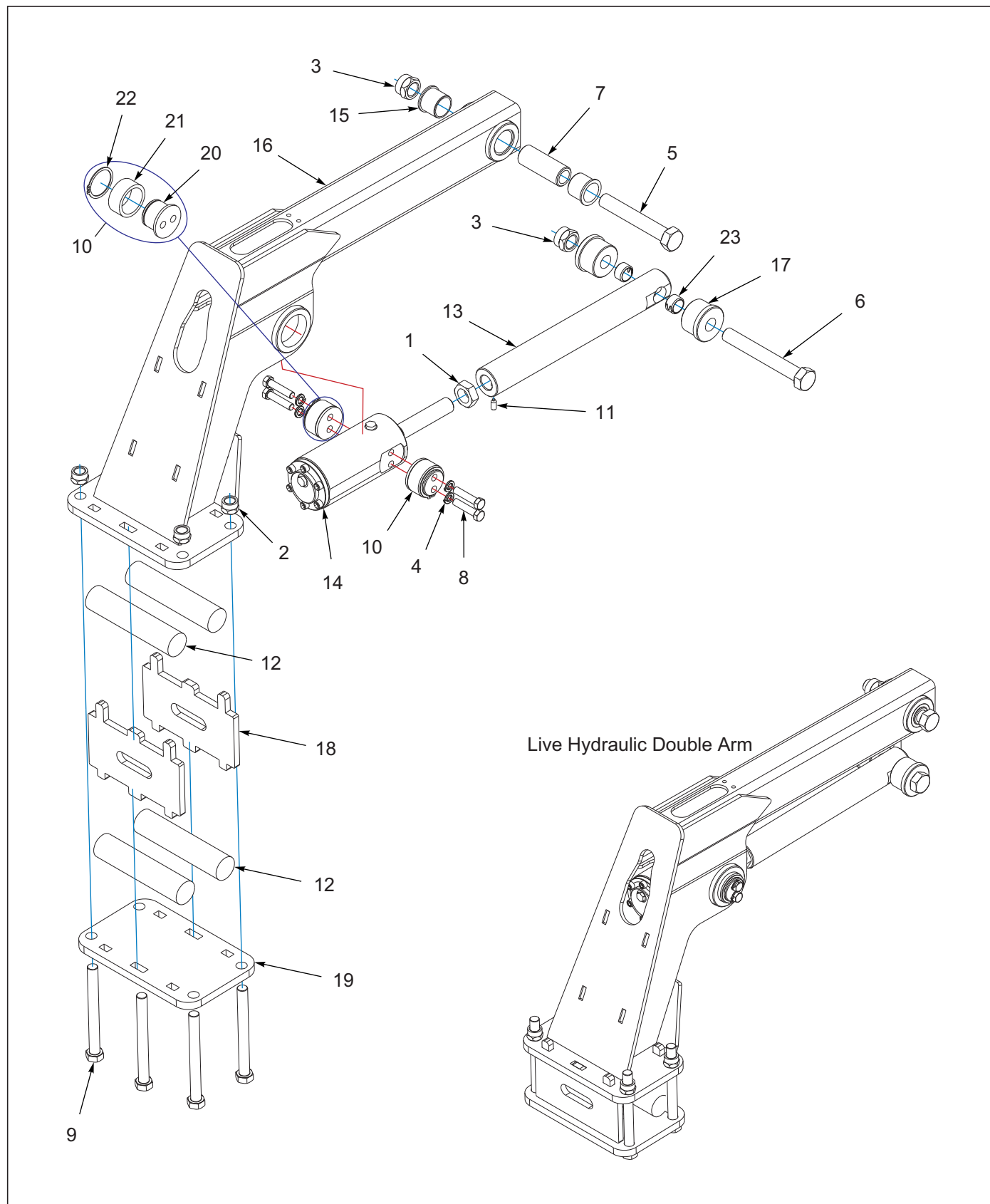
Figure 9-18: Live Hydraulic Double Arm Assembly
