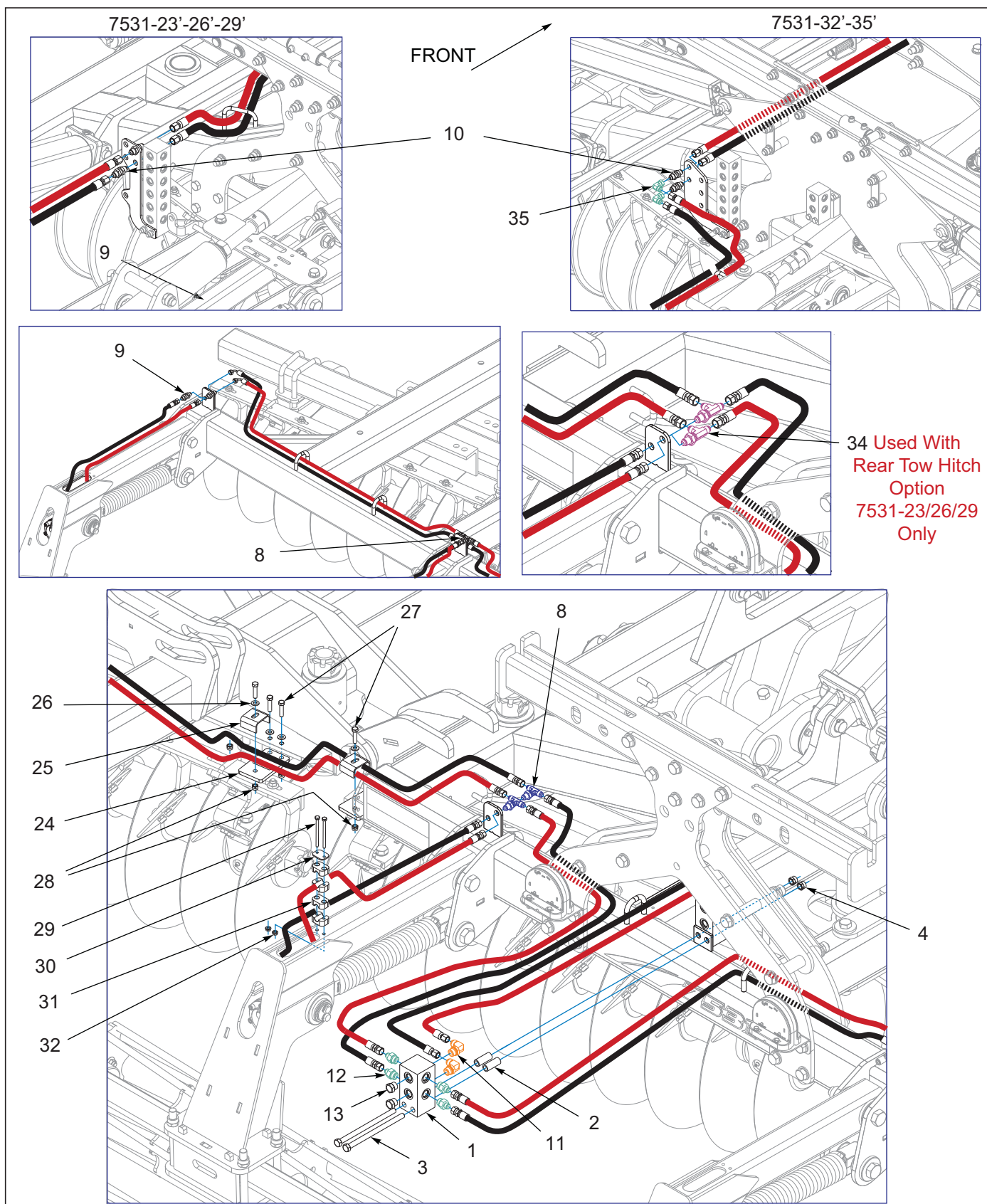
Figure 9-31: Reel Hydraulic Assembly (2 of 2)
