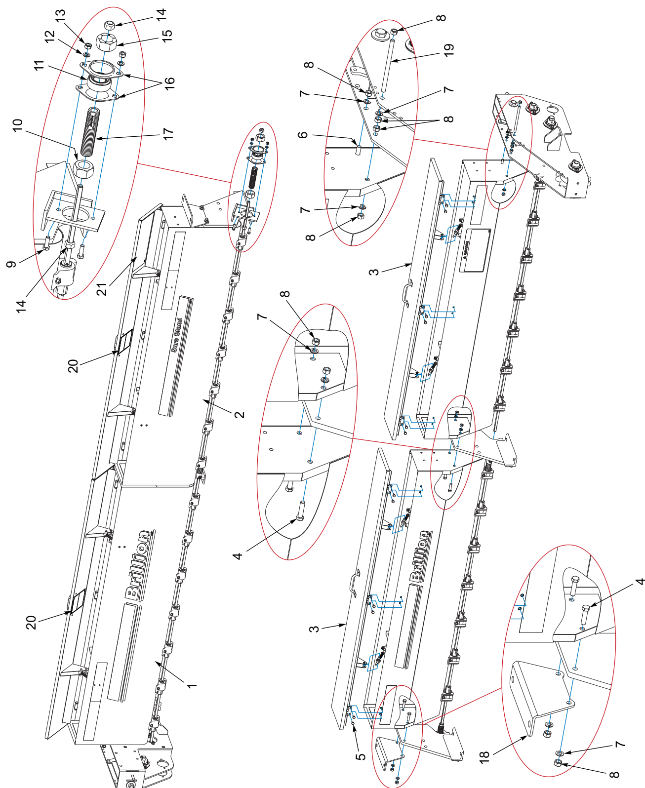
Figure 1-29: Front Seed Box (BEFORE 08/2025)
