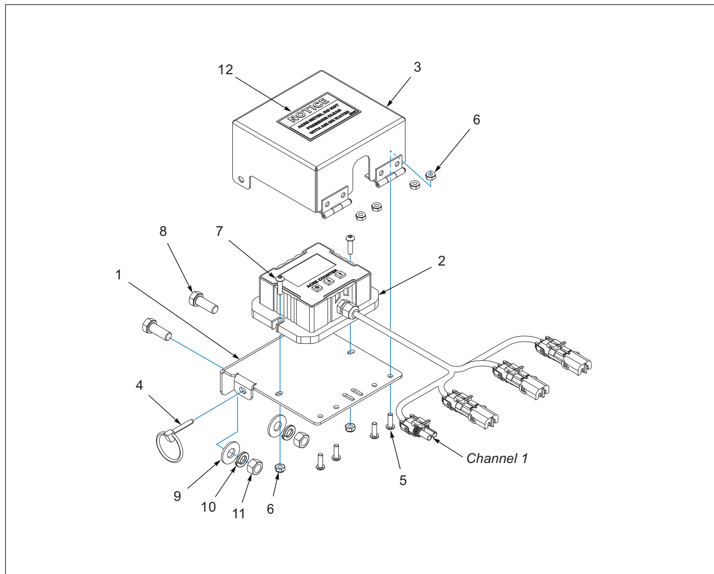
Figure 1-73: Acre Meter Assembly (AFTER 06/01/2025)
