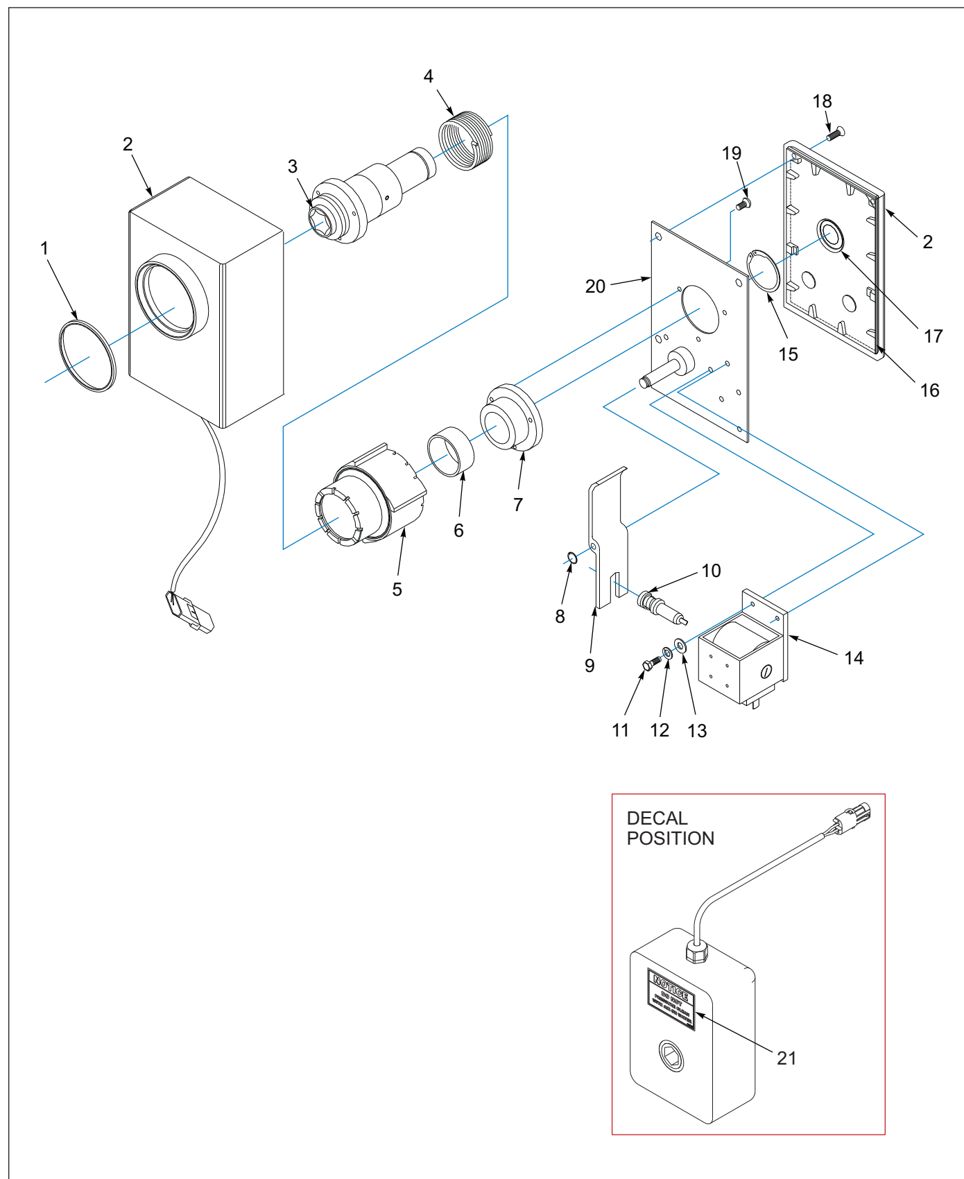
Figure 1-26: Electric Clutch - Optional
