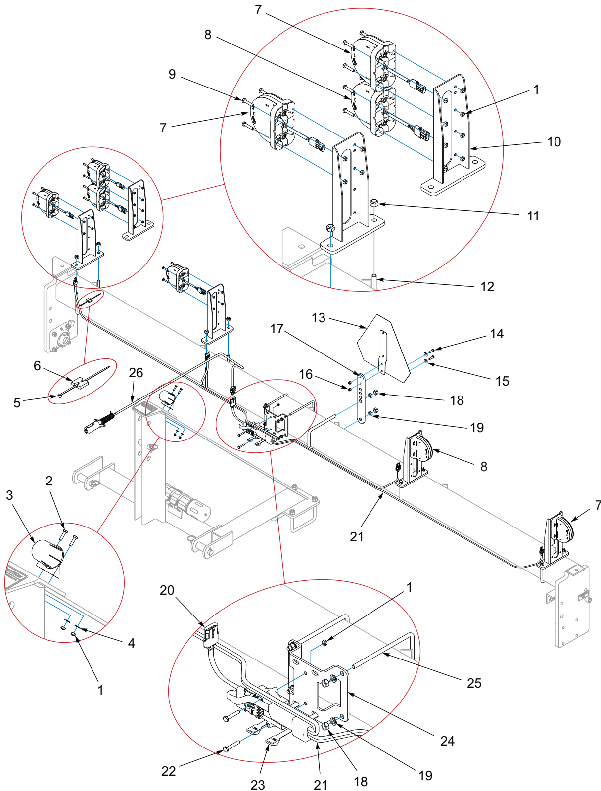
Figure 1-54: LED Warning Lamps - SD, 3-PT (09/2013 TO 08/2025)
